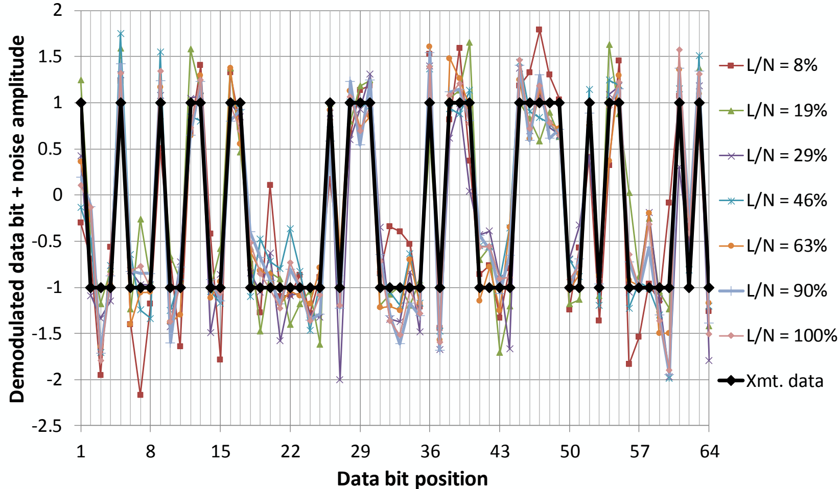
Plot of Demodulated Data Bit + Noise Amplitude
