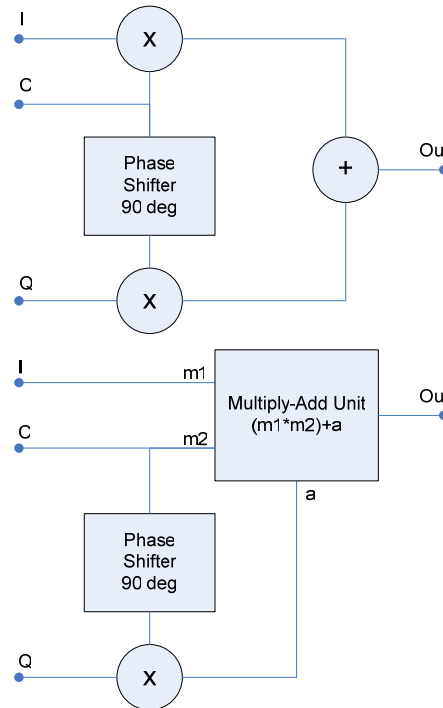
Figure 1 Functionally equivalent composite software modules.
